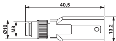
Plug M8 x 1, Y-distributor
